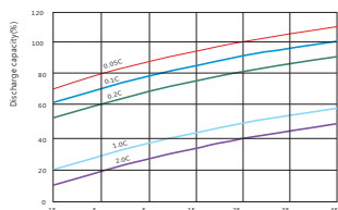
Discharge capacity vs. temperature
