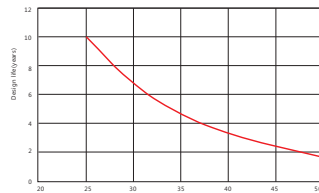
Design life vs. temperature
